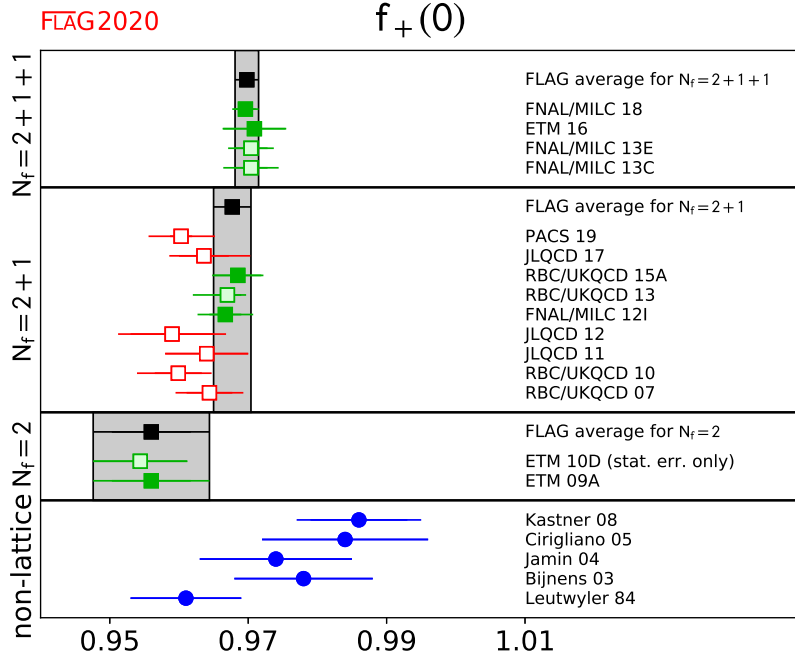
Figure 8: Comparison of lattice results (squares) for f_+(0) with various model estimates based on \chi PT [57, 59–62] (blue circles). The black squares and grey bands indicate our average (74)–(76). The significance of the colours is explained in Sec. 2.
